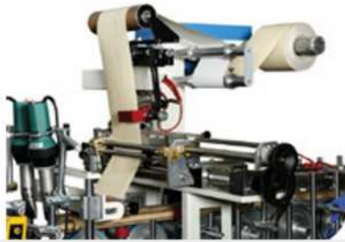
Folyo Kenar Kontrol Sistemi Special Foil Edge Control System For Perfect Routing
